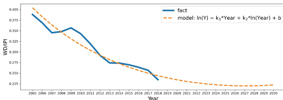
Fig. 11. The trend of changes in wastewater emissions/per unit of industrial production until 2030 Source: authors' calculations.
